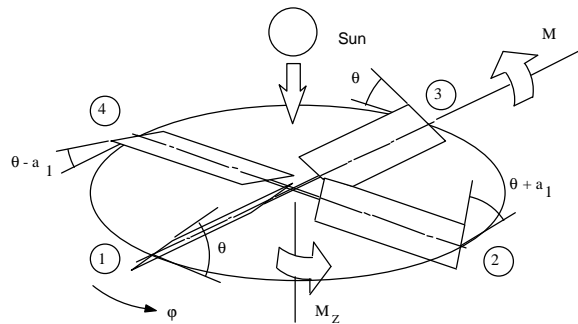
Figure 10. Cyclic Pitch Maneuver. 2
