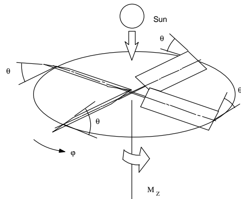
Figure 12. Collective Pitch Maneuver. 2
