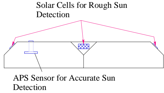
Figure 14. Solar Cell and APS Sun Sensor Locations.
