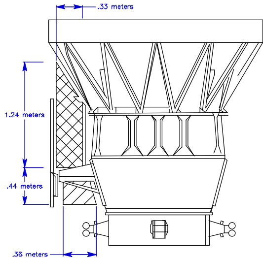
Figure 6. Usable Envelope for a Separating Secondary Payload, Three-Stage Mission.
