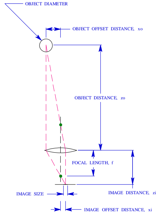
Figure 15. Geometry for sun direction determination.
