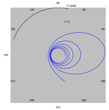
Figure 2. Earth Escape Trajectory for a Solar Sail With I = 5 .
