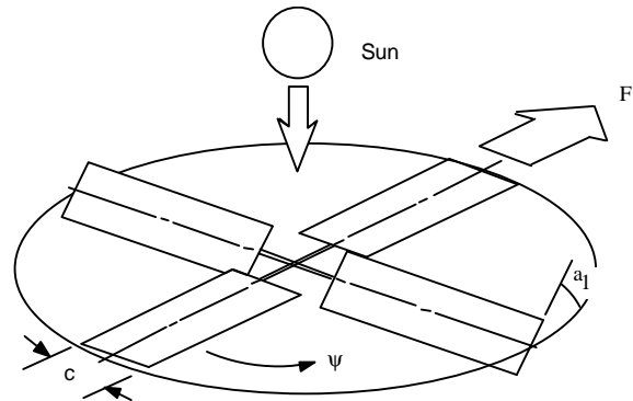
Figure 10. Cyclic Pitch Maneuver. 2
