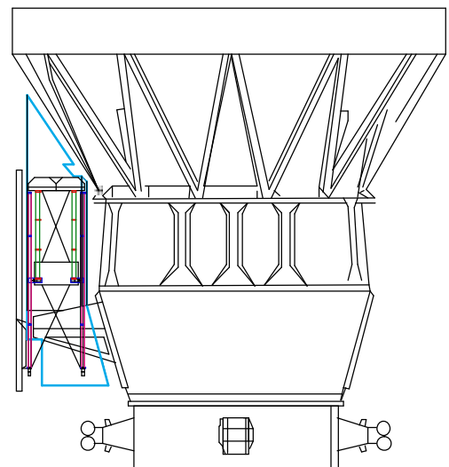
Figure 7. Solar Blade on Delta II.
