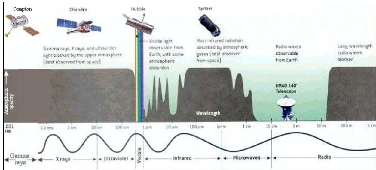
Figure 1. Atmospheric windows for power transmission in the micron range. Notice the narrow bands of high transmissivity near one micron.
