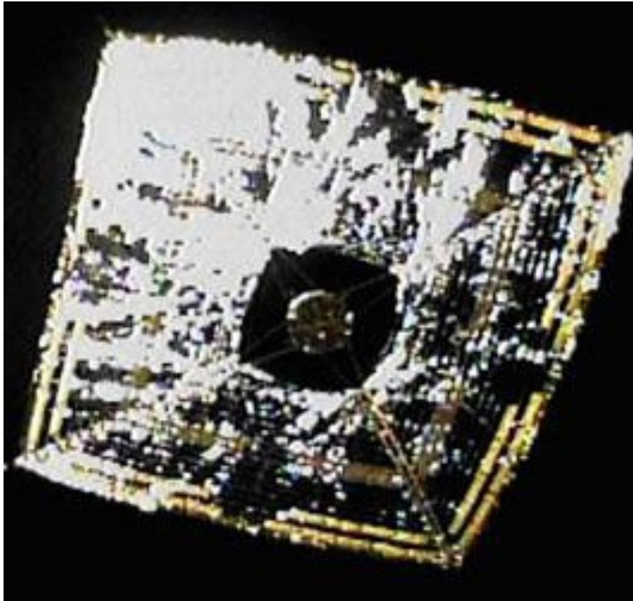
Figure 4. The Ikaros solar sail. Note the inner ring of faintly yellow materials. These are thin- \mu\text{m} solar cells. A PowerSat might employ this same design but extend the power production area to the entire sail. The more prominent yellow around the edge of the sail are liquid crystal devices used to control the satellite by electronically changing their reactivity. Image courtesy of JAXA.
